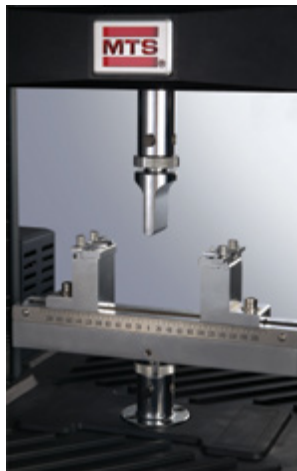
Bend Fixture
